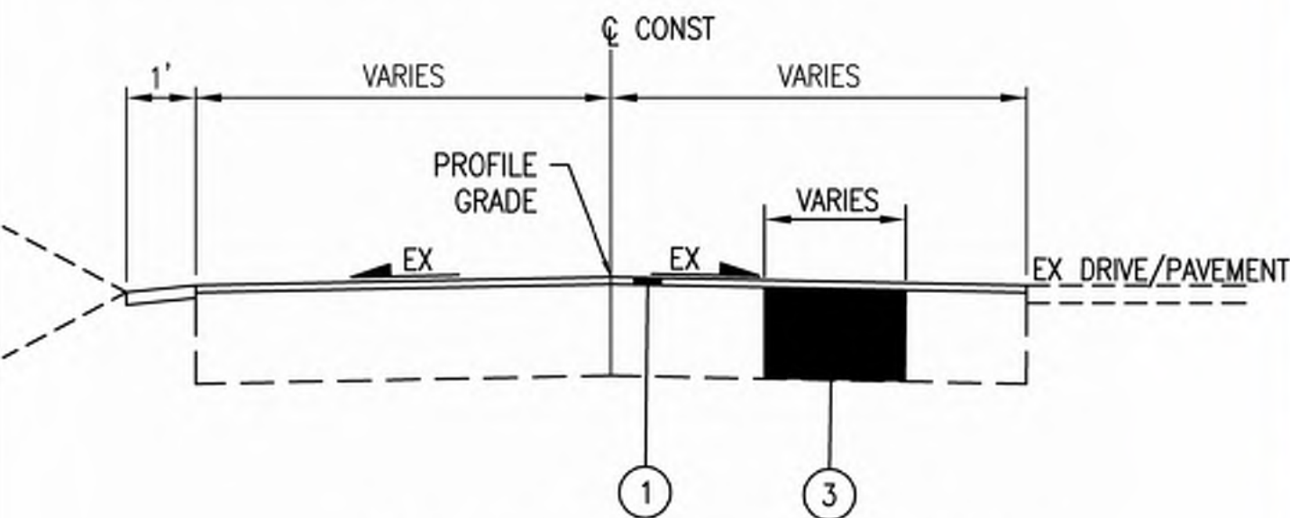
FULL DEPTH PAVEMENT REPAIR SECTION
